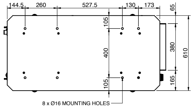
VIEW D
