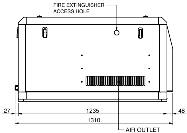
VIEW D
