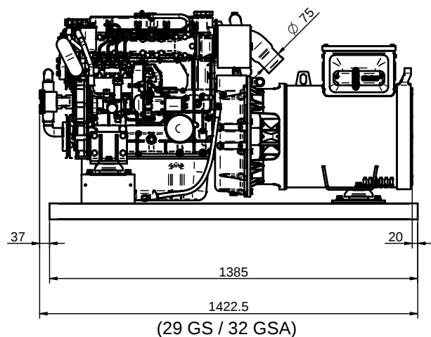
VIEW A
