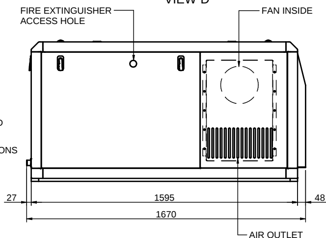
VIEW D
