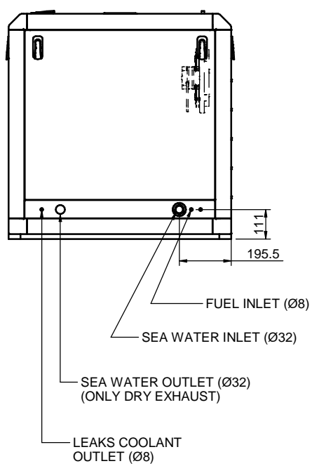
VIEW A
