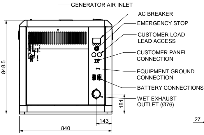
VIEW C
