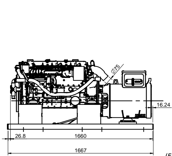
VIEW C
