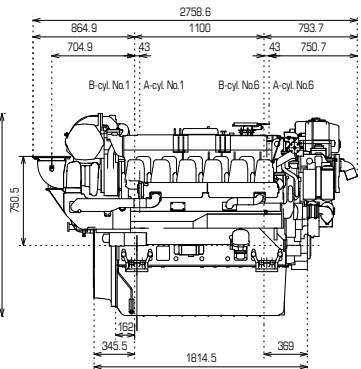
Engine only / Right side view
