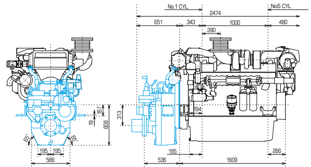
With YXH240 gear box / Rear view
