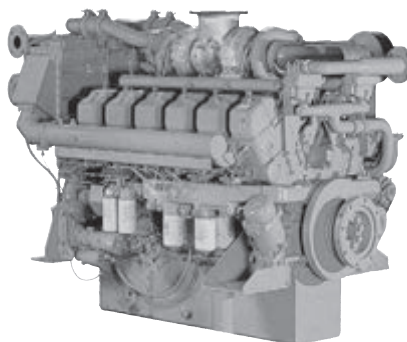
S12A2 MPTK 12-cylinder, 4-cycle, Water cooled, Diesel Engine Direct-injection, Turbocharged with Air-cooler Bore x Stroke (mm) : 150 x 160 Displacement (L) : 33.93
